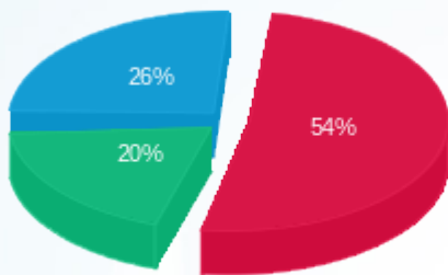
פסגה (53,576.70 Kwh) 54% גבע (19,457.60 Kwh) 20% שפל (25,727.90 Kwh) 26%
