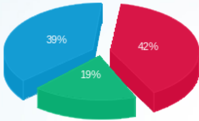
■ פסגה (122,120.74 Kwh) ■ גבע (55,002.02 Kwh) ■ שפל (114,221.16 Kwh)
