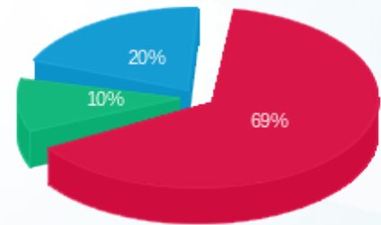
■ פסגה (8,091.90 Kwh) 69% ■ גבע (1,225.35 Kwh) 10% ■ שפל (2,376.85 Kwh) 20%
