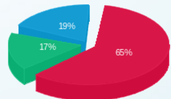
■ פסגה (43,133.07 kWh) 65% ■ גבע (11,070.68 kWh) 19% ■ שפל (12,612.12 kWh) 17%
