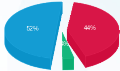
פסגה (135,514.11 ₪) גבע (10,779.80 ₪) שפל (159,298.48 ₪)
